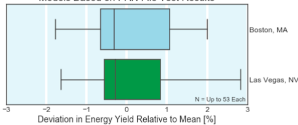
Spread of Predicted Annual Energy Yield Over Module Models Based on PAN File Test Results
