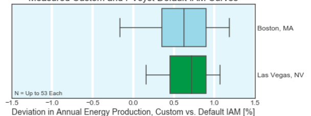
Spread of Deviations in Predicted Annual Energy Between Measured Custom and PVsyst Default IAM Curves
